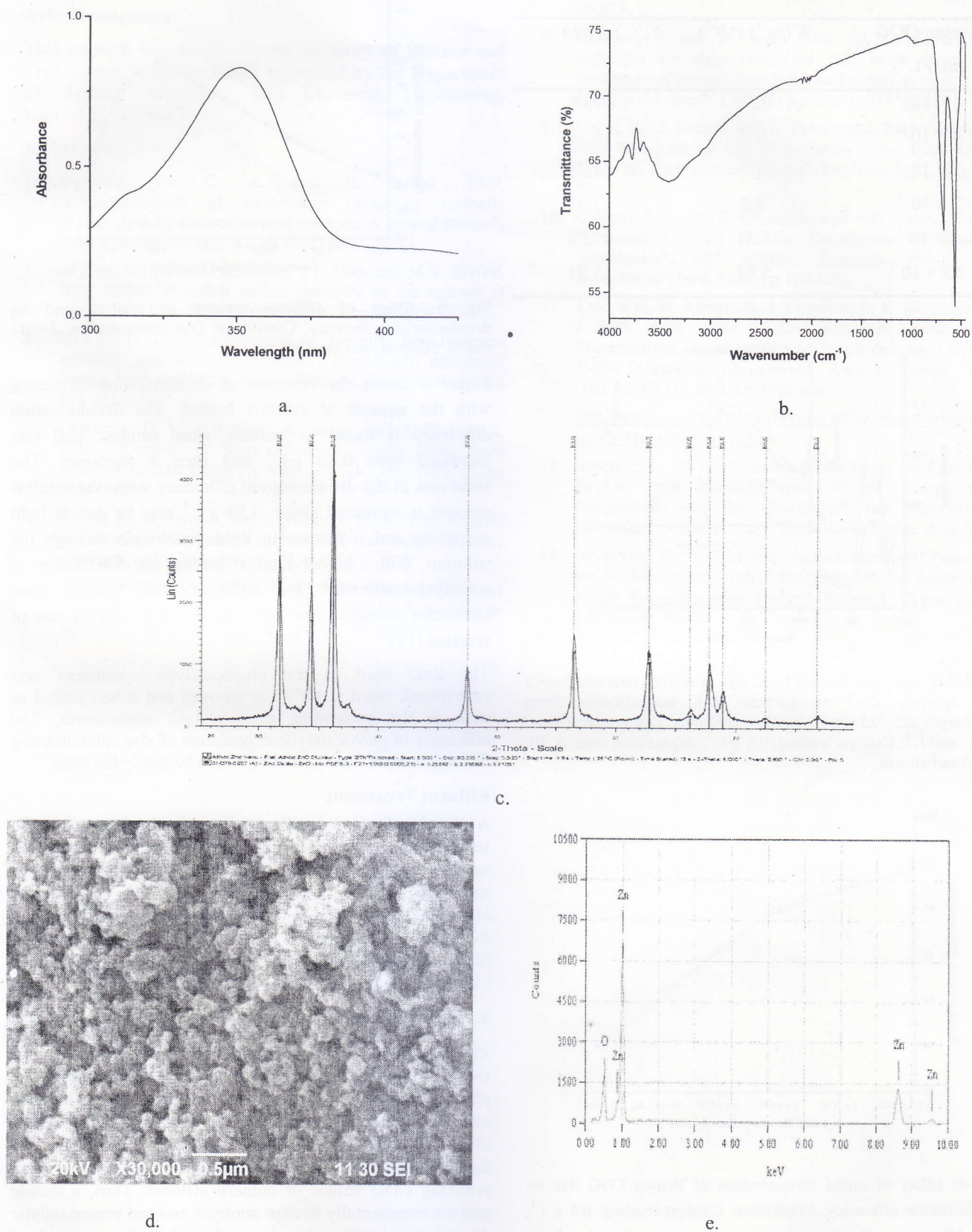
Fig. 2: Characteristics of prepared ZnO nanoparticle. a. UV-Visible; b. FT-IR; c. XRD d. SEM and e.EDX spectrum
