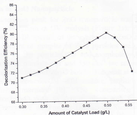
Fig. 5: Effect of different amount of catalyst load on decolorization efficiency. Conditions: Dye concentration, 2 × 10 -5 mol·L -1 ; degradation time, 40 min.
