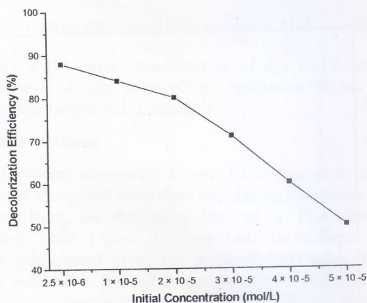
Fig. 4: Effect of initial concentration of Brown CGG dye on decolorization efficiency. Conditions: Catalyst loading, 0.5 g l -1 ; degradation time, 40 min.
