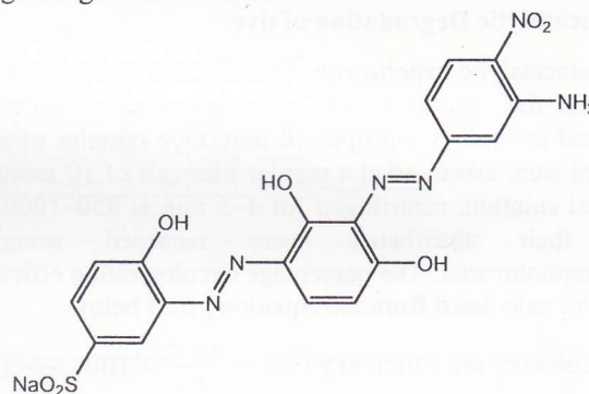
Fig. 1: Chemical structure of Brown CGG.
